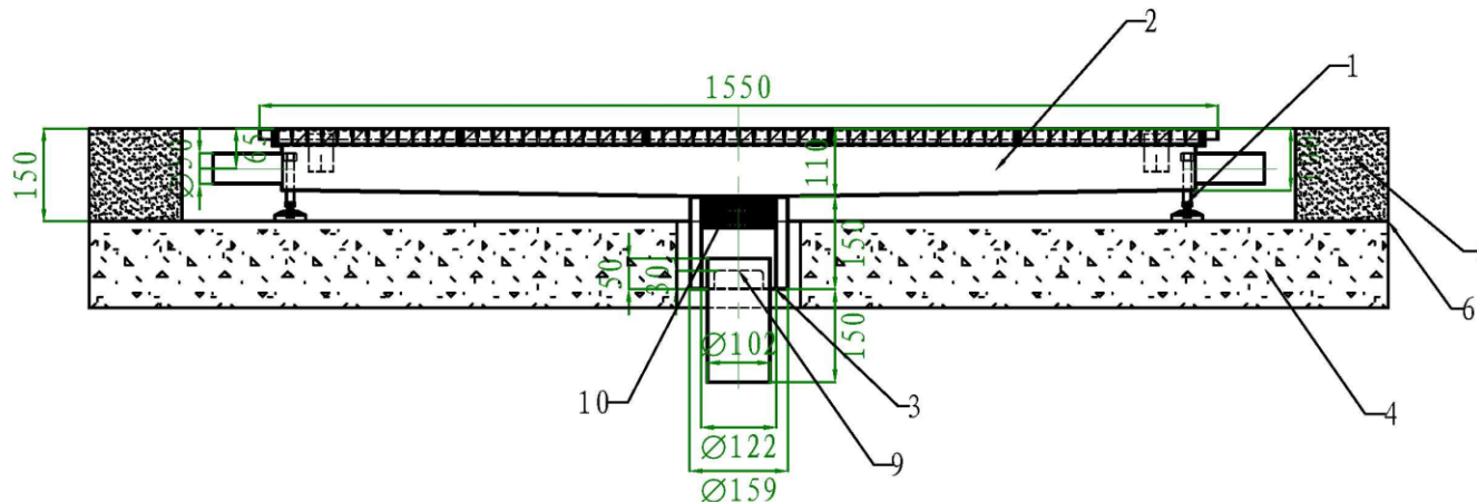
TYPICAL DETAIL OF FLOOR CHANNEL WITH GRATING & GULLY(WITH VERTICAL OUTLET)
