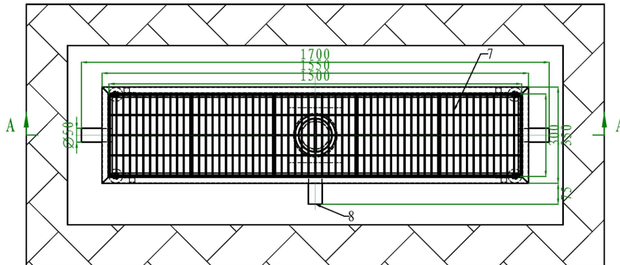
TYPICAL DETAIL OF FLOOR CHANNEL WITH GRATING & GULLY(WITH VERTICAL OUTLET)
